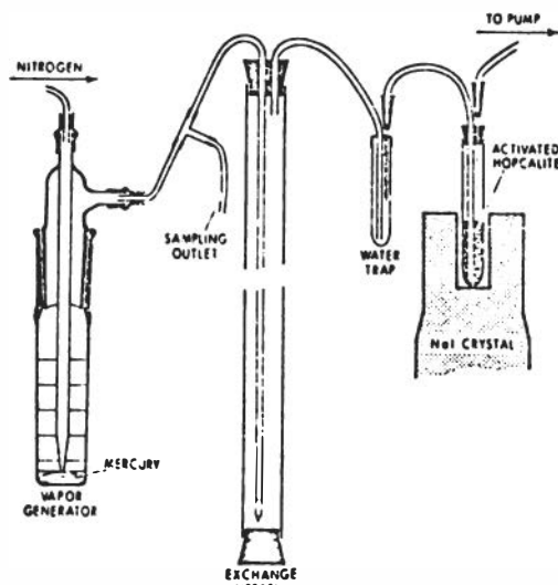
Figure 61. The exchange and counting assembly.
