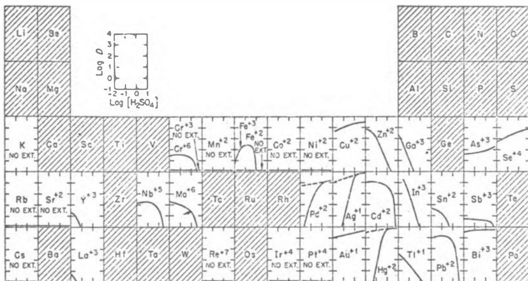
Figure 12. Extraction of metal ions from H_2SO_4 with di-n-butyl phosphorothioic acid •
