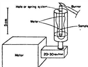
Figure 48. Sketch illustrating the quartz tube sealing technique.
