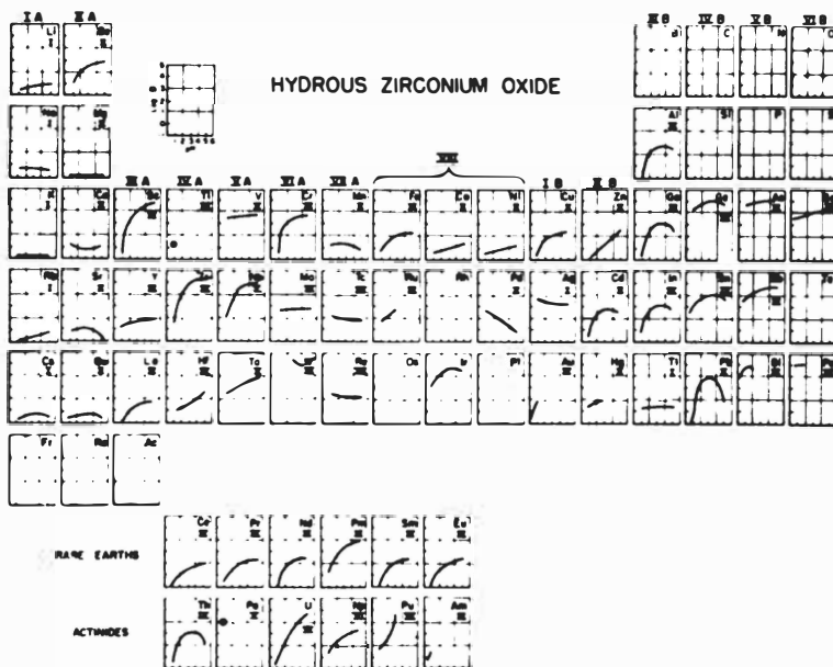
Figure 27. Exchange characteristics of elements on hydrous zirconium oxide.
