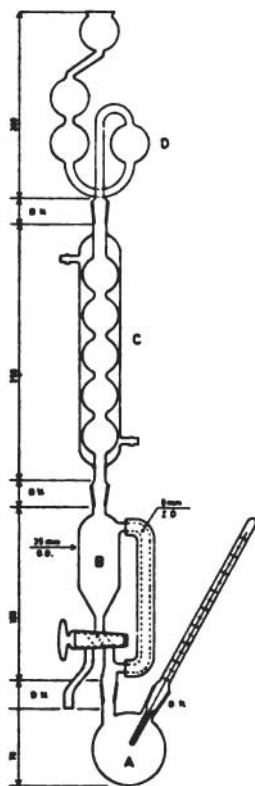
Figure 49. Apparatus for controlled decomposition of organic materials, also used as distillation apparatus.
