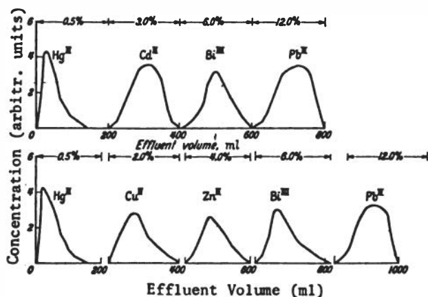
Figure 26. Elution of several cations with thiocyanate.
