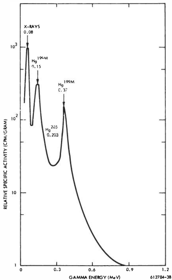
Figure 34. Gamma spectrum of neutron activated mercury of natural isotopic composition.
