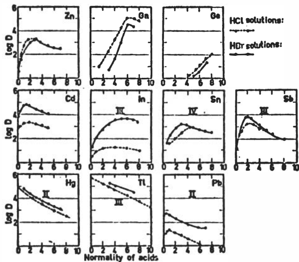
Figure 15. Adsorption of some elements with 18 electron configuration and of Sb(III), Pb(II) from HBr and HCl solutions.
