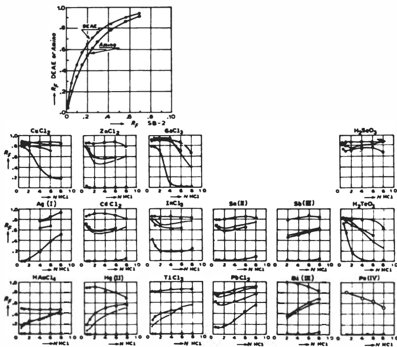
Figure 33. R_F values of metal ions on Whatman No. 1 paper ( \circ — \circ ), Sb-2 resin paper ( \blacksquare — \blacksquare ), DE-20 cellulose anion-exchange paper ( \bullet — \bullet ), and AE-30 cellulose anion-exchange paper ( \square — \square ) are plotted against the concentration of HCl. With the exception of Pt(II) which was placed below Pt(IV) the metal ions placed in their positions in the periodic table.
