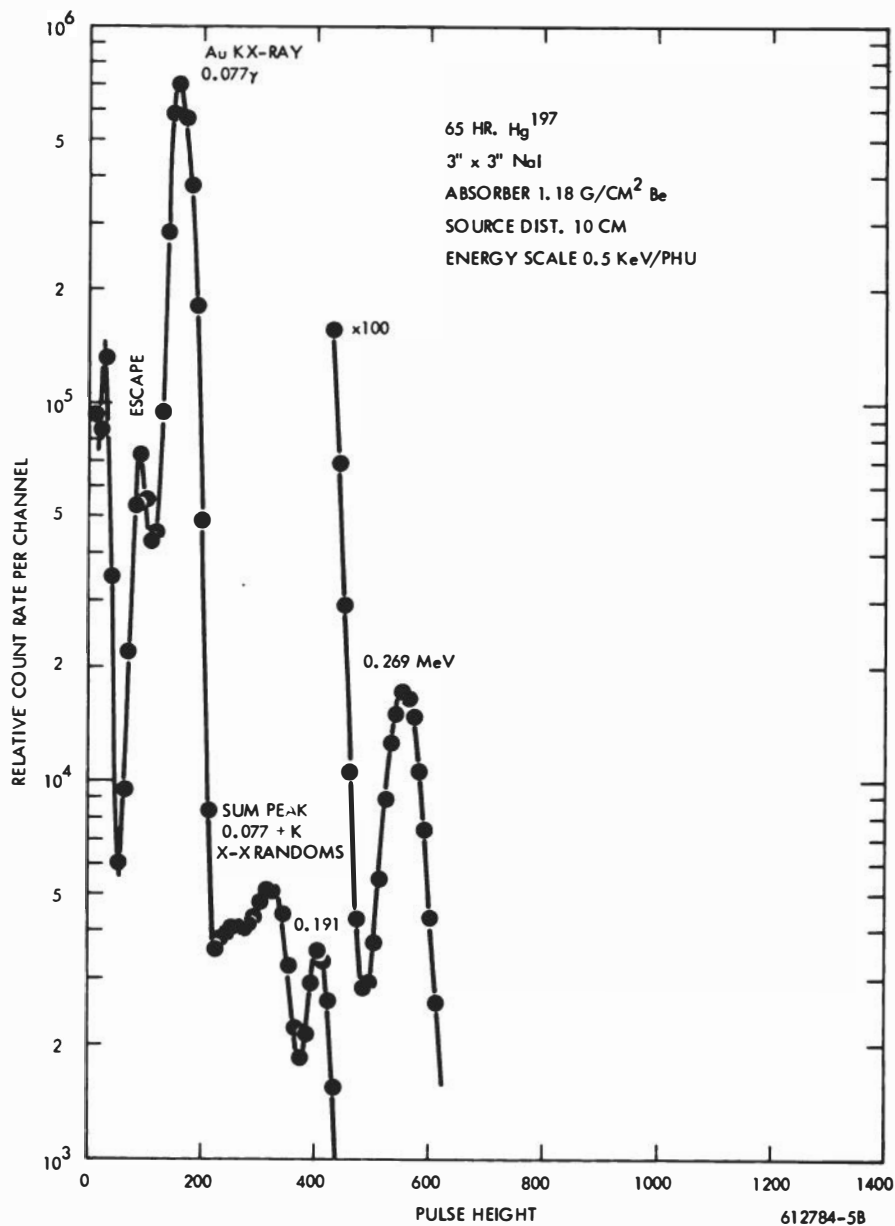
Figure 39. Gamma spectrum of 65-hour Hg^{197} .
