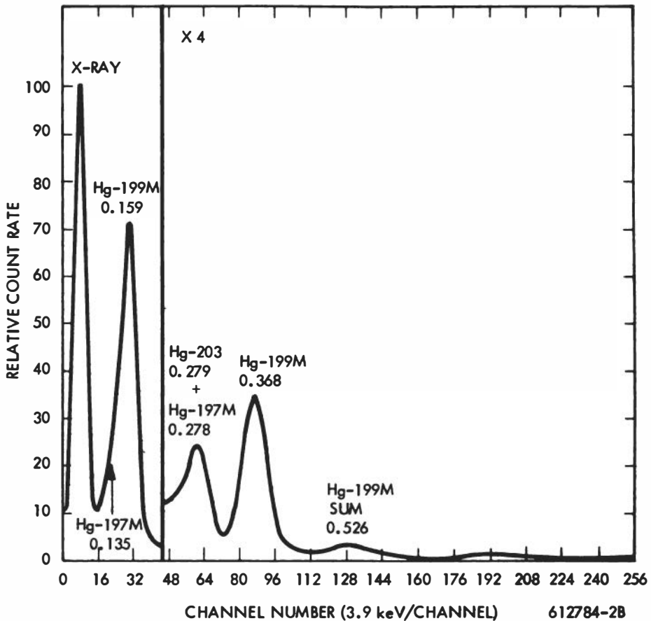
Figure 36. Gamma spectrum of natural mercury irradiated with 30 MeV photons.
