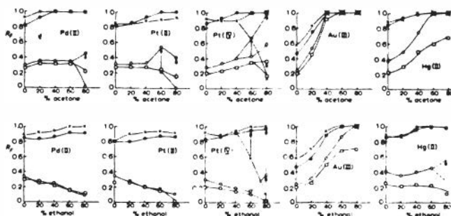
Figure 32. R_f values on some anionic chloro-complexes on various cellulose exchangers with acetone-2N HCl and ethanol-2N HCl mixtures. (□) Diethylamino ethyl cellulose, (○) Aminoethyl cellulose, (●) Whatman No. 1, (X) Cellulose phosphate)
