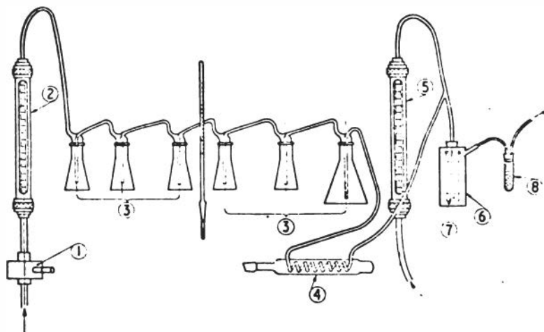
Figure 58. Details of the system for producing and sampling known concentrations of mercury vapor. (1) Flostat minor to regulate the air flow through the saturation system; (2) rotameter to measure the volume of the saturated air; (3) Quickfit wash bottles having mercury layer in the bottom; (4) coil condenser having mercury droplets in the coils; (5) rotameter to measure the volume of mercury-free air; (6) lead shield; (7) midget impinger; (8) absorber.
