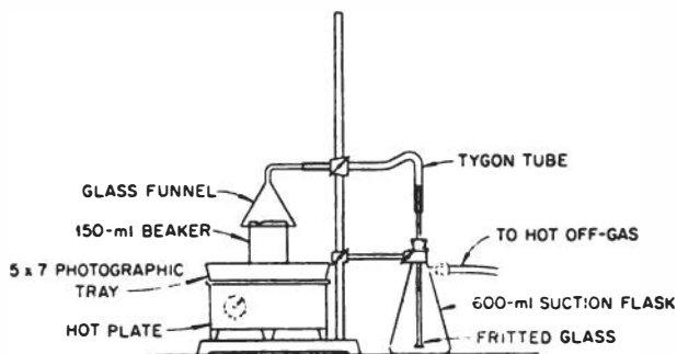
Figure 46. Hot Off-Gas Scrubber Unit.
