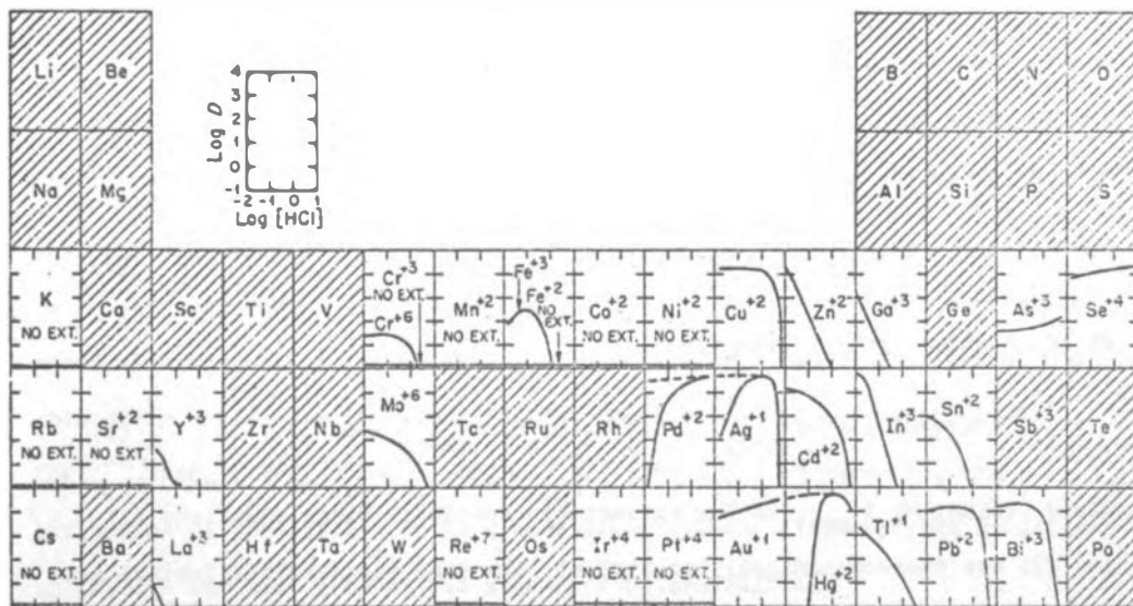
Figure 13. Extraction of metal ions from HCl with di-n-butyl phosphorothioic acid •
