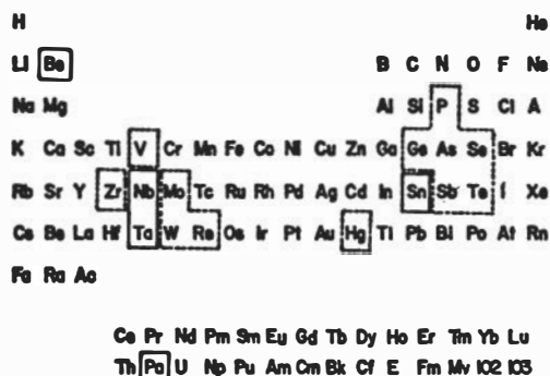
Figure 6. Elements extracted in fluoride system. Solid blocks--appreciably extracted; broken blocks--partially extracted.
