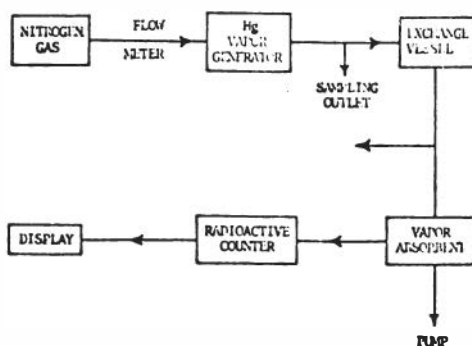
Figure 60. Schematic arrangement of apparatus.
