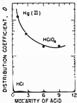
Figure 23. Distribution coefficients for \text{Hg(II)} as a function of acid molarity.
