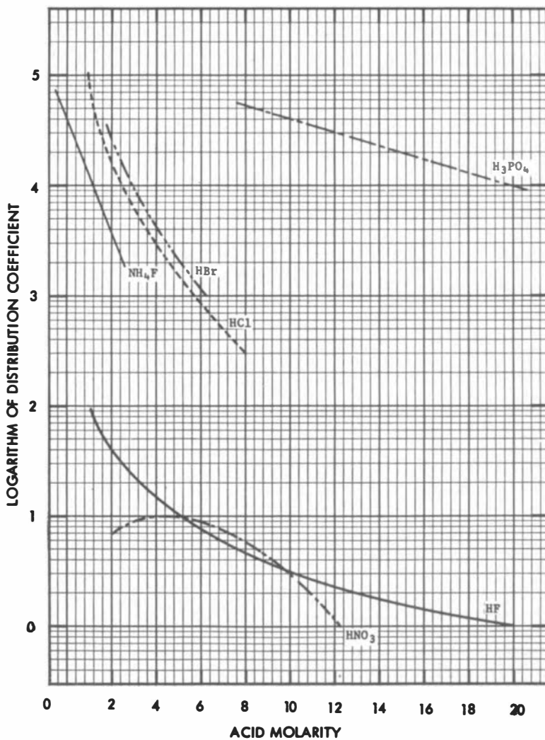
Figure 63. Elution behavior of Hg(II) from Dowex-1 as a function of acid molarity and anion.
