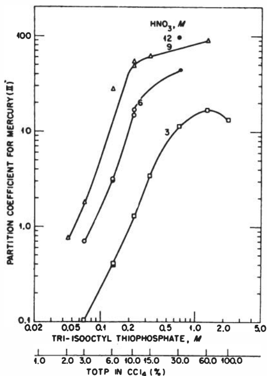
Figure 11. Partition coefficient of \text{Hg(II)} as a function of reagent concentration for various concentrations of \text{HNO}_3
