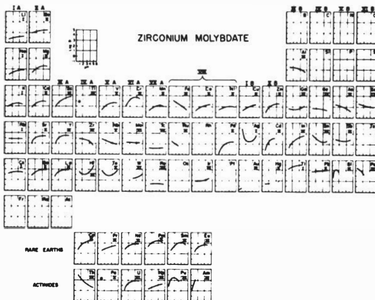
Figure 28. Exchange characteristics of elements on zirconium molybdate.
