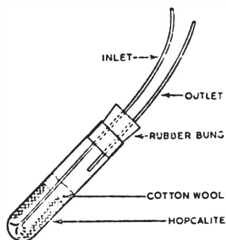
Figure 57. The absorber.
