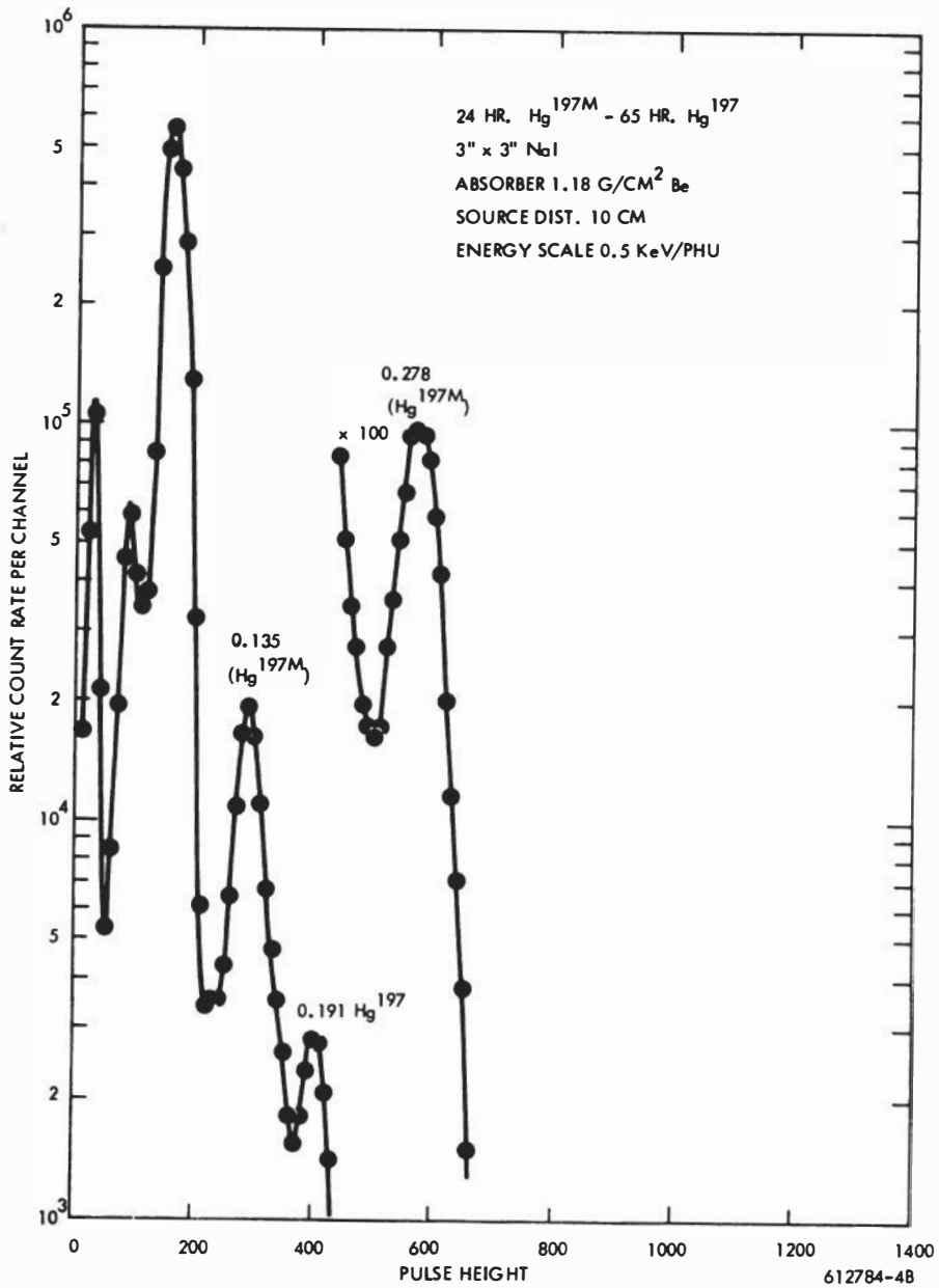
Figure 38. Gamma spectrum of the parent-daughter pair 24-hour \text{Hg}^{197\text{m}} -65-hour \text{Hg}^{197} .
