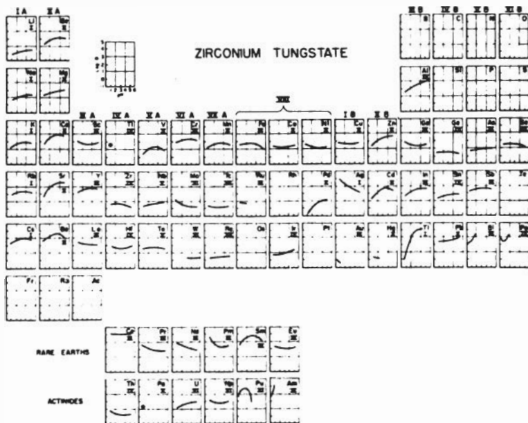
Figure 30. Exchange characteristics of elements on zirconium tungstate. (M-8).
