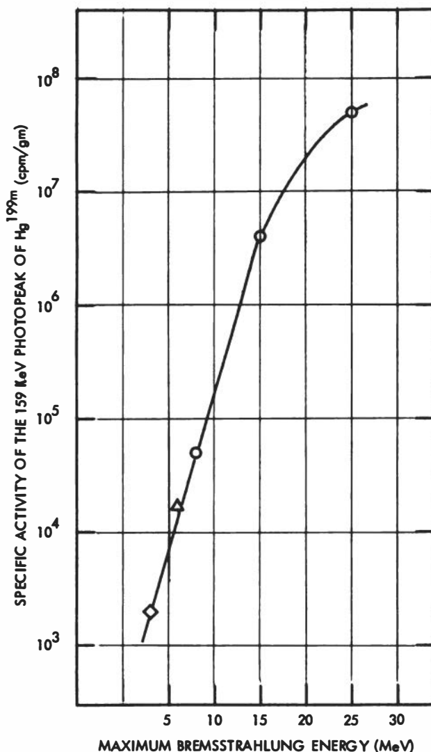
Figure 35. Yield of the 159 keV photopeak of Hg 199m as a function of the maximum incident bremsstrahlung energy. (◊ taken from Ref. 175, △ Ref. 176, and ○ Ref. 228).
