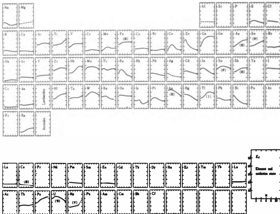
Figure 9. Dependence of the distribution ratio K_D on normality of HCl in the 1% TBPO system.
