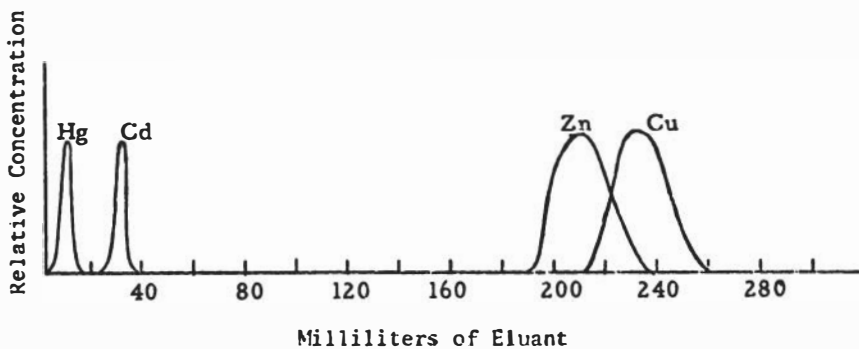
Figure 24. Elution sequence of \text{Hg} , \text{Cd} , \text{Zn} , and \text{Cu} from a Dowex 50-X4 column.
