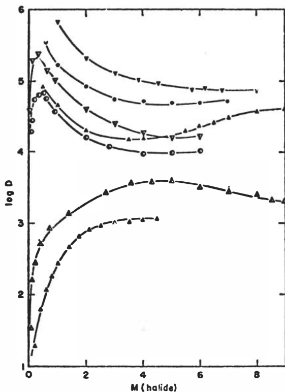
Figure 16. Distribution coefficients ( \log D ) of mercury (filled points), cadmium (half-filled points) and zinc (empty points) vs. halide molarity: \Delta lithium chloride, \circ sodium bromide, and \nabla sodium iodide solutions.
