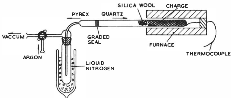
Figure 56. Apparatus for heating the Hg/Ag/Cu alloy.
