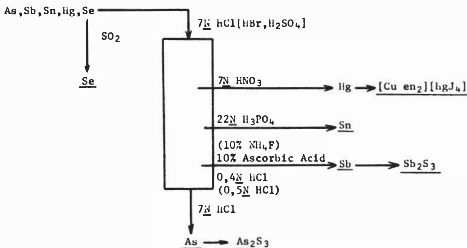
Figure 54. Flowchart for the separation of As, Sb, Sn, lig and Se.
