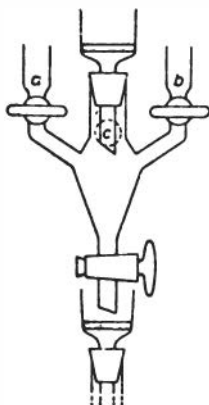
Figure 44. Filtration Element; a, b, sidearms for the addition of reagents, c to be connected to a vacuum line.
