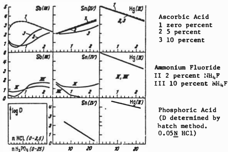
Figure 53. Dependence of distribution coefficients on acid molarity.
