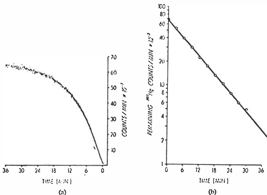
Figure 62. (a) Recorder tracing. (b) Semi-log plot. The radioactivity remaining in the solution at any time was calculated from the pen-recording as described in the text.
