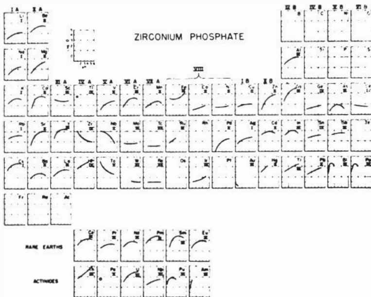
Figure 29. Exchange characteristics of elements on zirconium phosphate.
