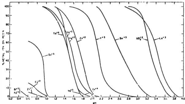
Figure 25. Retention of different metal ions by Dowex-50 resin as a function of pH of solutions containing EDTA.
