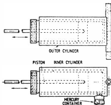
Figure 59. Plane (upper sketch) and side view (lower sketch) of the 1.0\ \mu\text{g} calibrator.
