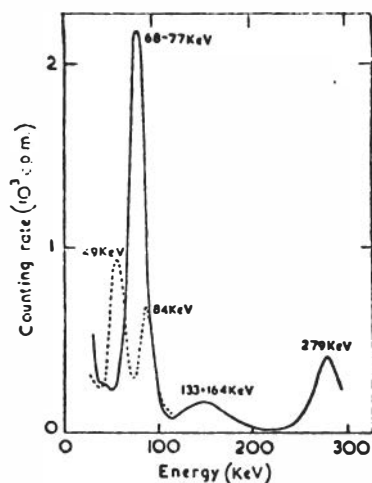
Figure 43. \gamma -Ray spectrum of Hg 197+197m (full line), and of Tm 170 (broken line).
