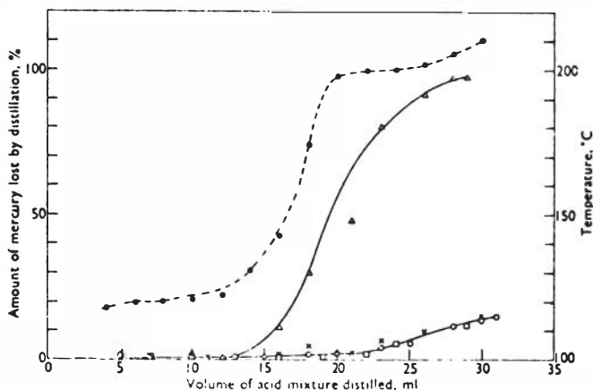
Figure 41. Loss of mercury by distillation when acid mixture was heated under different conditions; X, acid mixture alone; O, acid mixture with 1 ml of concentrated hydrochloric acid; □, acid mixture in stream of carbon dioxide; Δ, acid mixture with 0.5 g of glycine. The broken line curve, O, is the temperature-volume distilled curve for the nitric-perchloric-sulphuric acid mixture.
