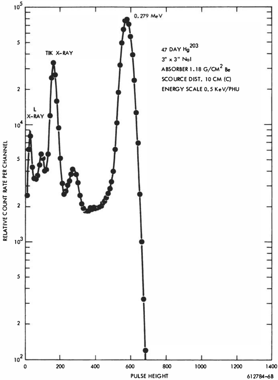
Figure 40. Gamma spectrum of 47 day Hg^{203} .
