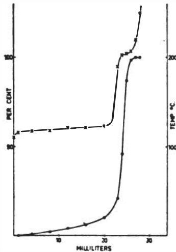
Figure 50. Distillation curve for mercury. (% of mercury distilled, X Temperature of Fumes) See page 201 for copyright citation.
