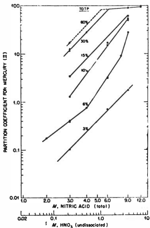
Figure 10. Partition coefficient of \text{Hg(II)} from aqueous \text{HNO}_3 solutions at various concentrations of TOTP
