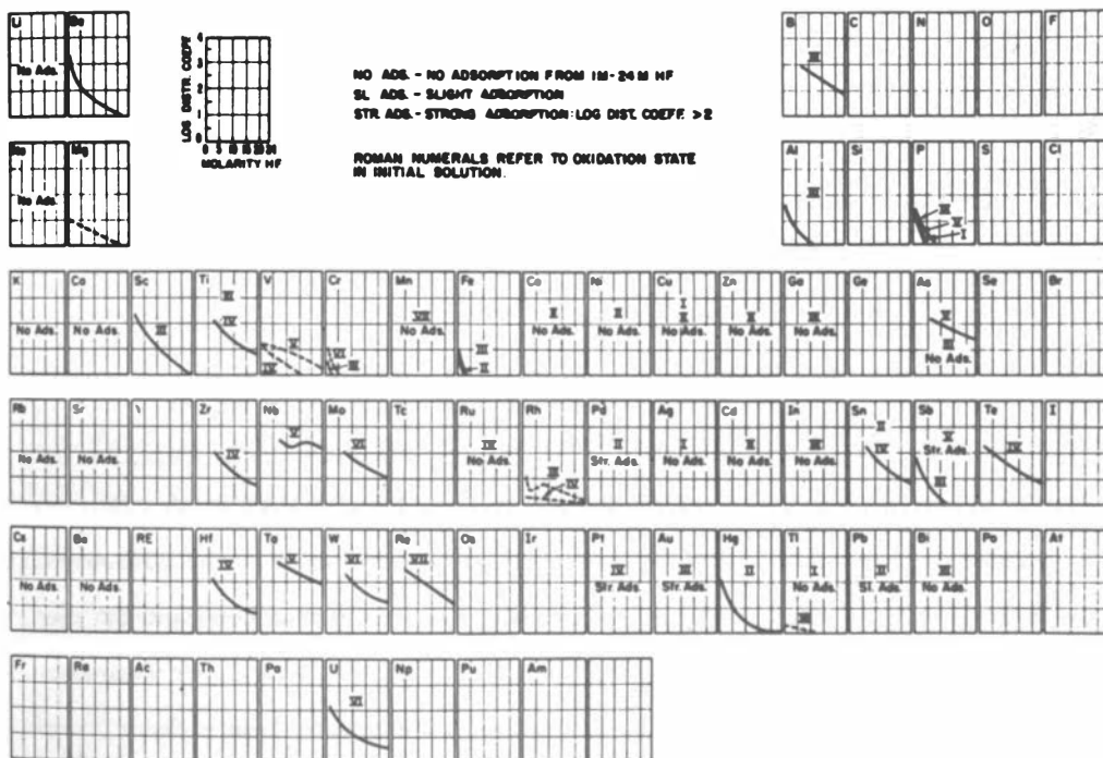
Figure 17. Removal of elements from solution in 1M to 24M hydrofluoric acid with 200-mesh anion exchange resin.
