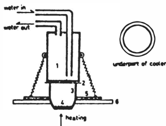
Figure 55. Apparatus for Hg distillation. 1, cooler: made of brass (o.d. ~3 cm, o.h. ~5 cm); 2, Ag plate (thickness ~0.05 mm, diam. ~3 cm); 3, nickel crucible (i.d. ~2.7 cm, height ~2.5 cm); 4, sample deposited on copper powder (Cu ~1g); 5, iron crucible-supporter; 6, asbestos.
