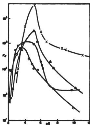
Figure 20. Variation of the distribution coefficient for mercury with pH and tartrate concentration. \odot - in 8.5 \cdot 10^{-2} M tartrate; \square - 4.25 \cdot 10^{-2} M tartrate; \triangle - in 2.12 \cdot 10^{-2} M tartrate; \times - in 2.12 \cdot 10^{-3} M tartrate.
