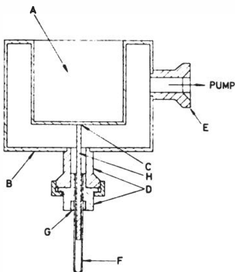
Figure 47. Vacuum evaporation apparatus for mercury separations.
