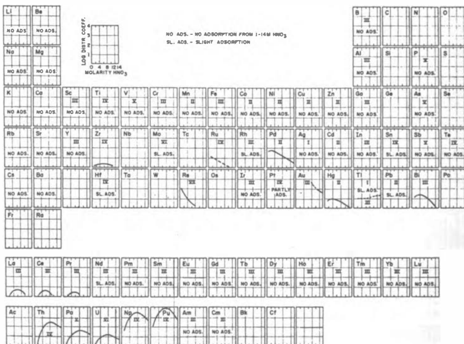
Figure 18. Removal of elements from solution in 1M to 14M nitric acid with a strongly basic anion-exchange resin.
