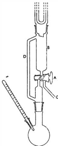
Figure 42. Apparatus for controlled decomposition of organic material.
