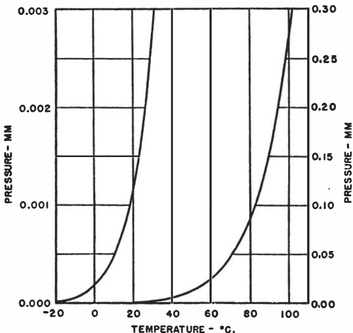
Figure 2. Vapor pressure curve of mercury (pressure in mm. of mercury). See page 201 for copyright citation.
