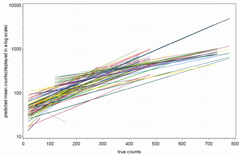
FIGURE B-8 Individual laboratory estimated calibration functions for PCM. NOTE: The y-axis is in a log scale with base = 10.
