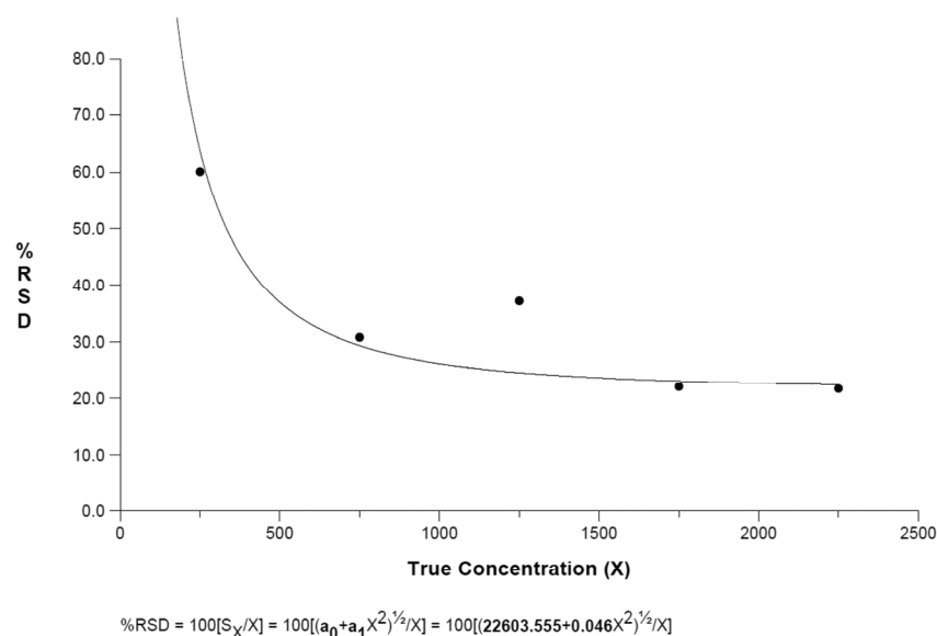
FIGURE B-5 Percent relative standard deviation vs. concentration for asbestos TEM samples in \text{mm}^2 .
