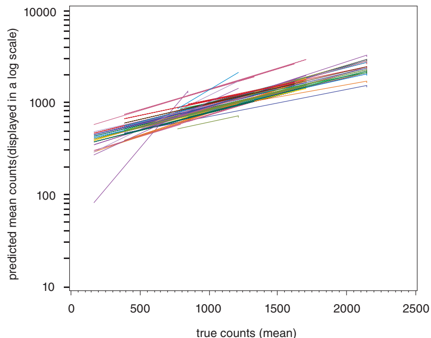
FIGURE B-2 Individual laboratory estimated calibration functions. NOTE: The y-axis is in a log scale with base = 10.
