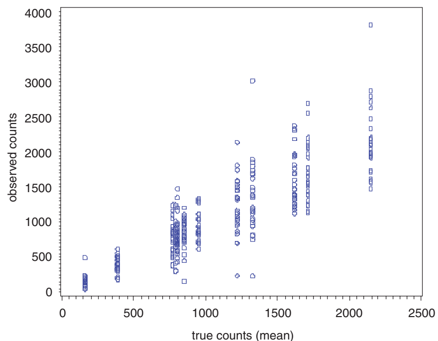
FIGURE B-1 Raw asbestos (AM) counts analyzed by TEM.
