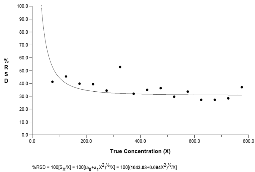
FIGURE B-11 Percent relative standard deviation vs. concentration for asbestos PCM samples in \text{mm}^2 .
