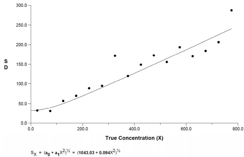
FIGURE B-10 Standard deviation vs. concentration for asbestos PCM samples in \text{mm}^2 .
