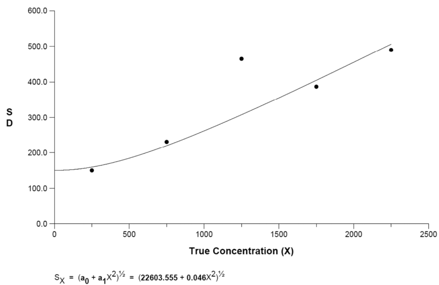
FIGURE B-4 Standard deviation vs. concentration for asbestos TEM samples in \text{mm}^2 .
