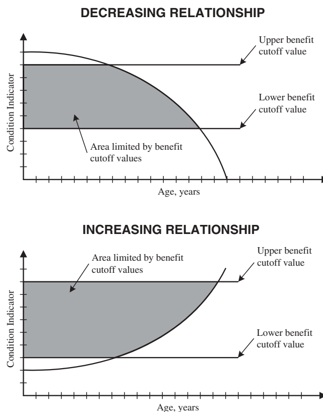
Figure 2. Illustration of the application of upper and lower benefit cutoff values on both decreasing and increasing condition indicators for the do-nothing case.
