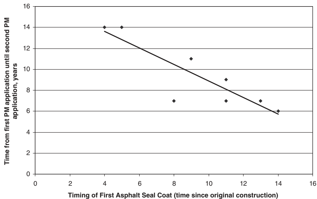
Figure 31. General trend between the life of the first preventive maintenance treatment and its application timing (time after initial construction).
