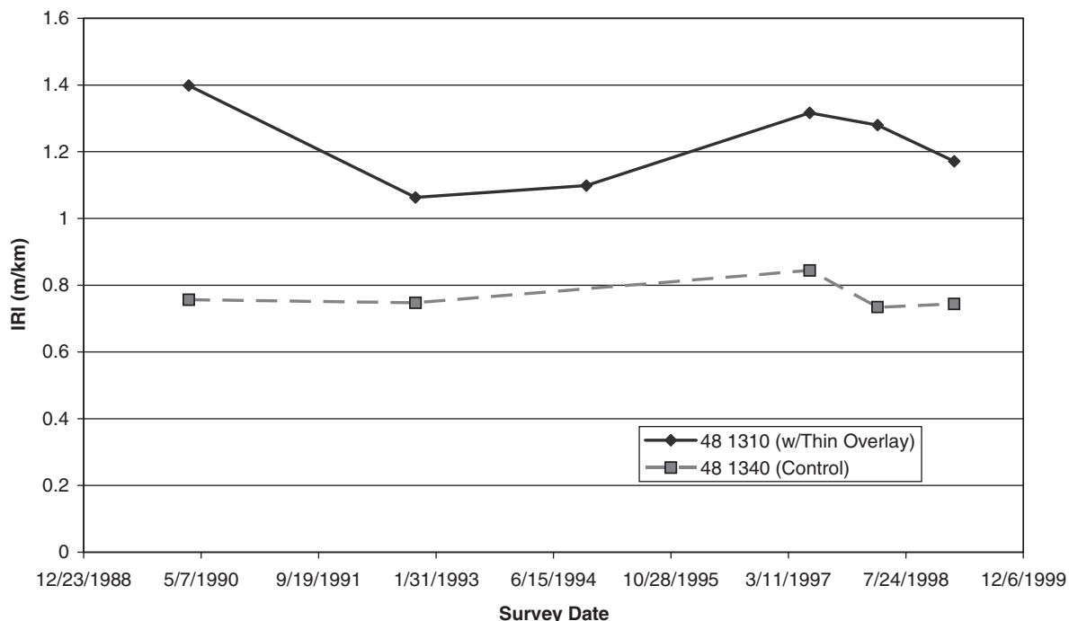
Figure 34. Example of LTPP data exhibiting a counterintuitive trend for a thin overlay application.
