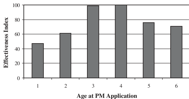
Figure 11. Example of Effectiveness Index versus timing of preventive maintenance application.
