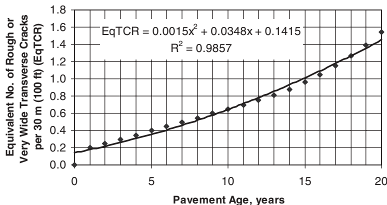
Figure 23. Estimated do-nothing curve for Case Study 2—Kansas.
