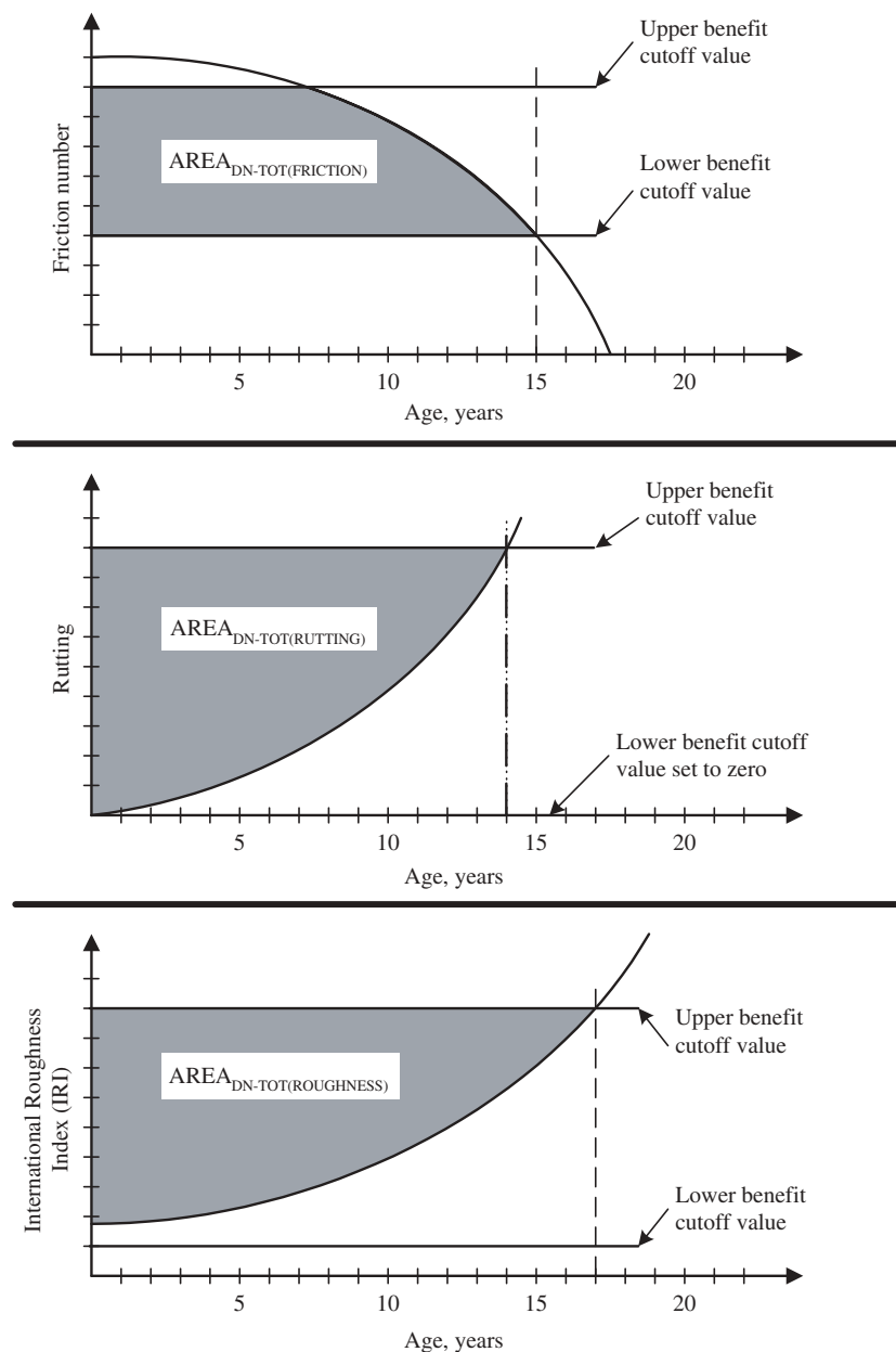
Figure 4. Total areas associated with individual condition indicators for the do-nothing options.
