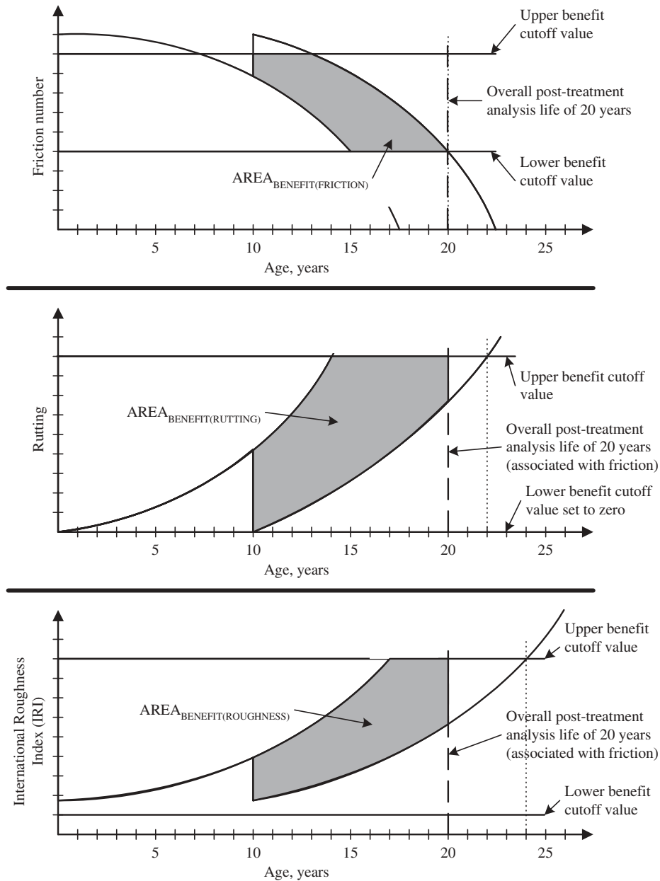
Figure 10. Illustration of benefit areas associated with individual post-treatment condition indicators (applicable for investigating multiple condition indicators).
