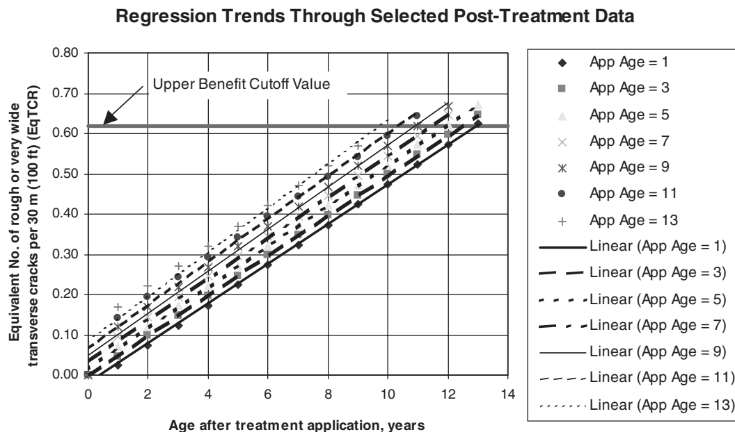
Figure 24. Illustration of post-treatment performance relationships based on KDOT models.
