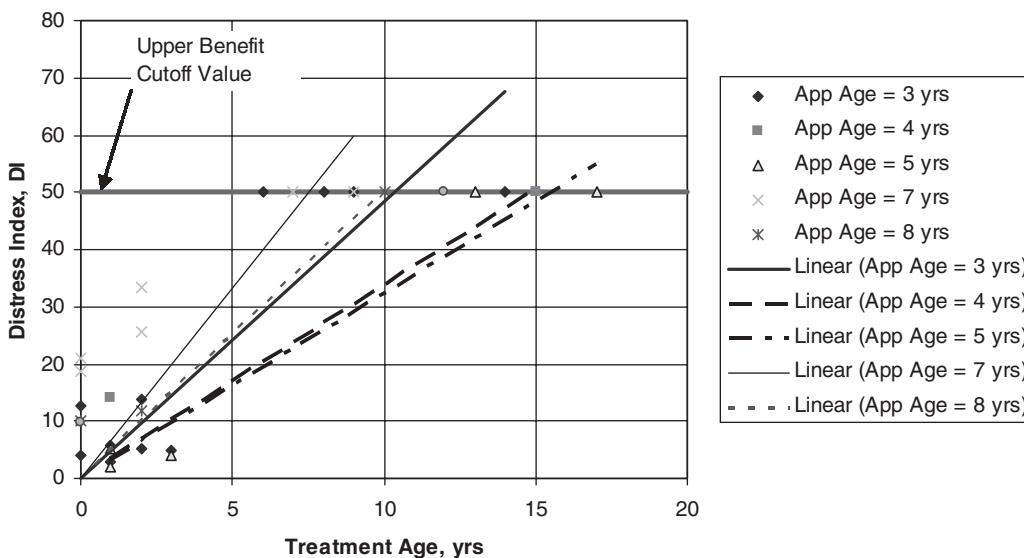
Figure 28. Post-treatment performance trends for bituminous crack sealing applied at different ages.
