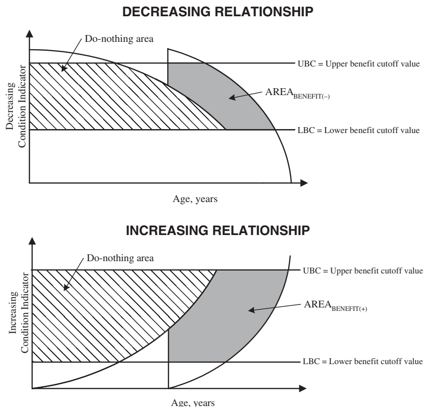
Figure 9. Illustration of the benefit area ( AREA_{BENEFIT} ) for a single decreasing or increasing individual post-treatment condition indicator.
