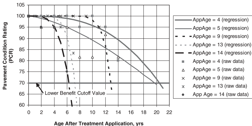
Figure 32. Determined post-treatment performance relationships for Case Study 4—North Carolina.
