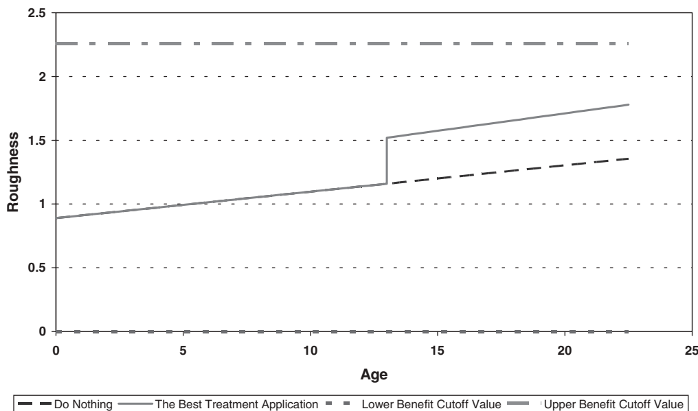
Figure 21. Roughness versus age for the most appropriate application age of 13 years for Case Study 1—Arizona.
