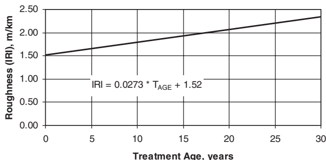
Figure 16. Assumed post-treatment seal coat roughness relationship for Case Study 1—Arizona.
