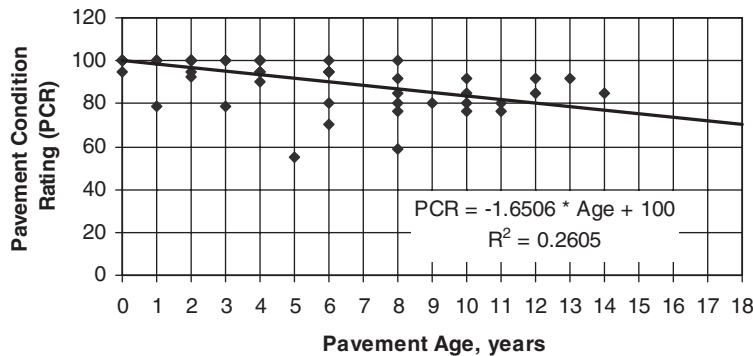
Figure 30. Assumed representative do-nothing curve for the North Carolina projects.
