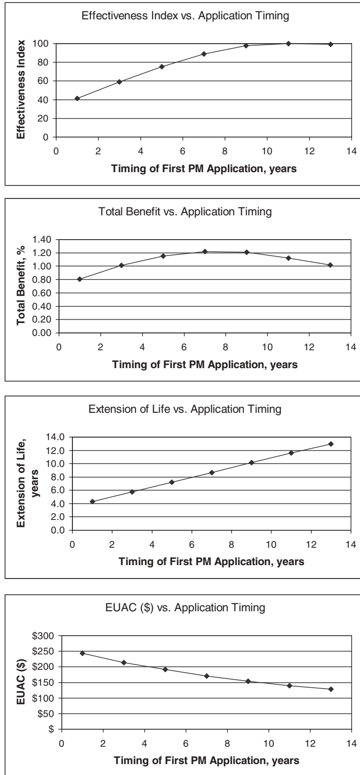
Figure 25. Summary charts for Case Study 2—Kansas.
