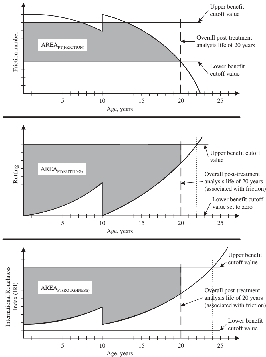
Figure 8. Illustration of the total areas associated with individual condition indicators.
