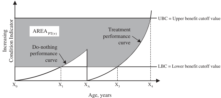
Figure 7. Determination of total areas associated with decreasing and increasing individual condition indicators.
