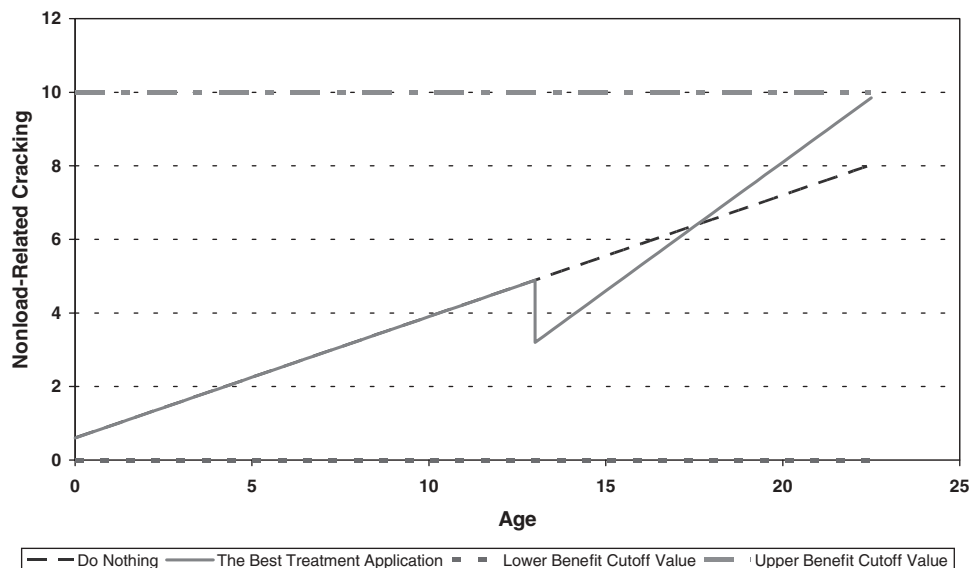
Figure 20. Cracking versus age for the most appropriate application age of 13 years for Case Study 1—Arizona.
