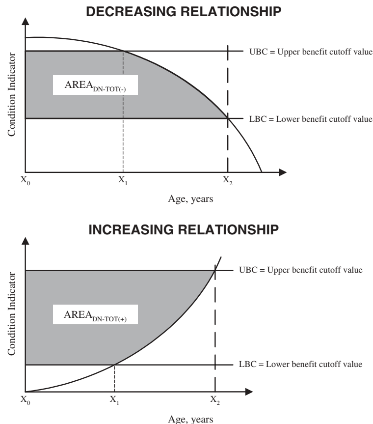
Figure 3. Total areas associated with decreasing and increasing condition indicators for do-nothing options.
