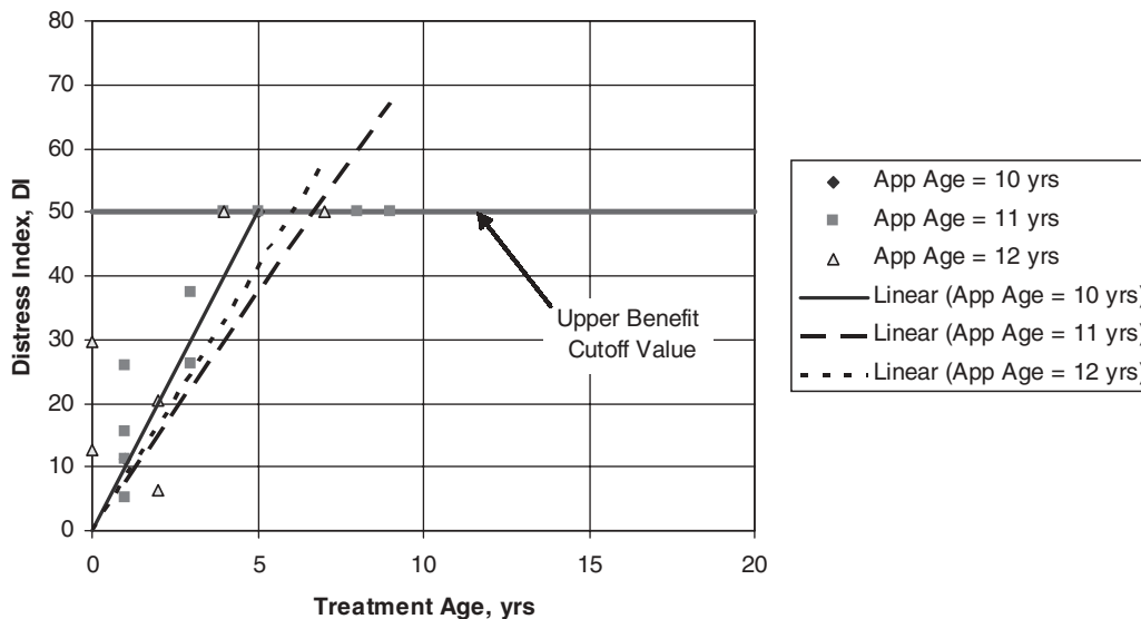
Figure 27. Post-treatment performance trends for chip seals applied at different ages.
