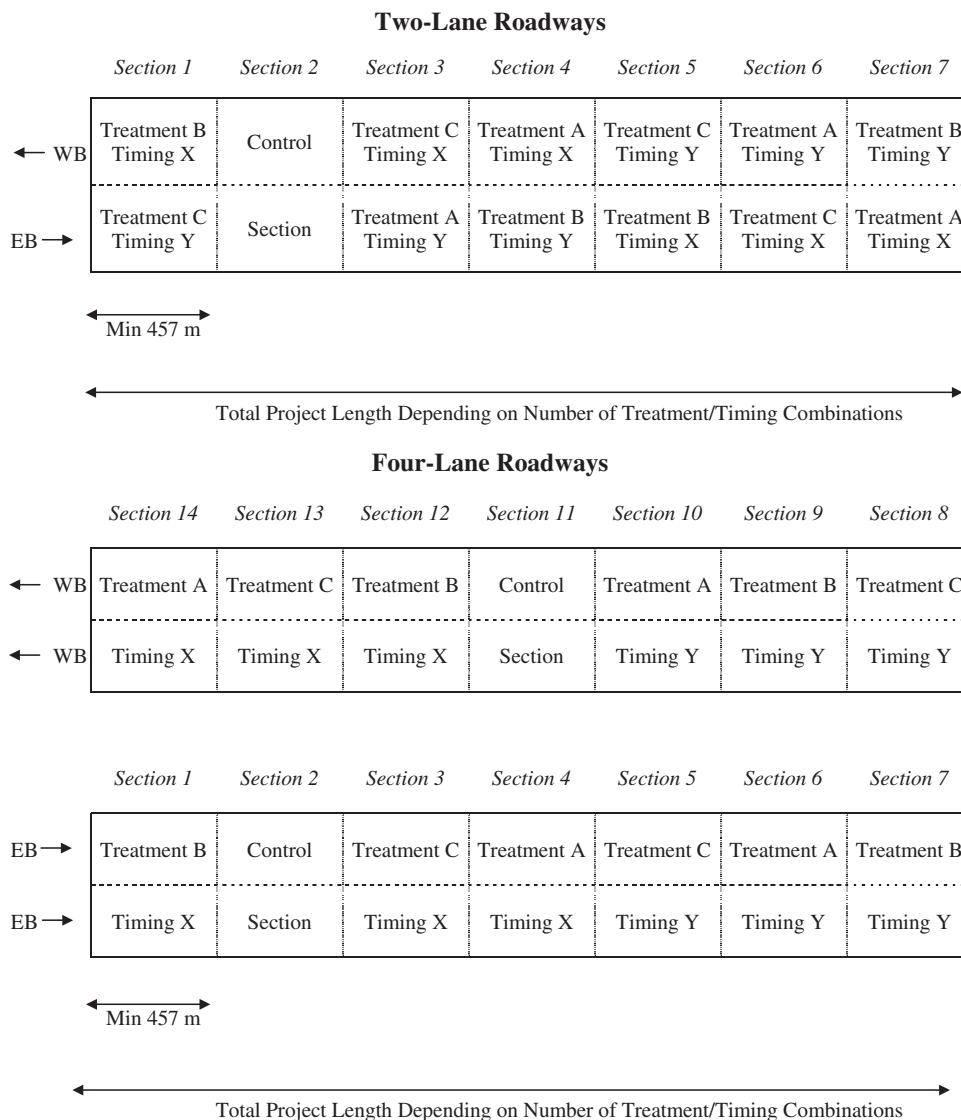
Figure D-1. Example test section layouts for 2-lane and 4-lane roadways.
