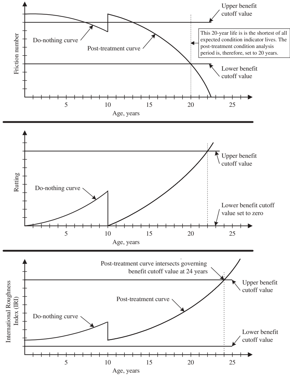
Figure 6. Determination of the overall post-treatment condition expected service life (analysis period).
