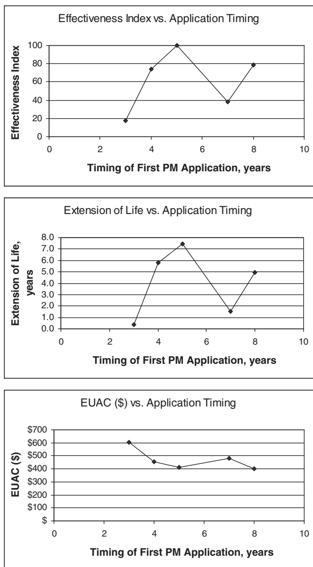
Figure 29. Summary charts of crack sealing for Case Study 3—Michigan.
