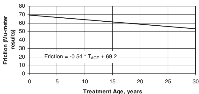
Figure 17. Assumed post-treatment seal coat friction relationship for Case Study 1—Arizona.
