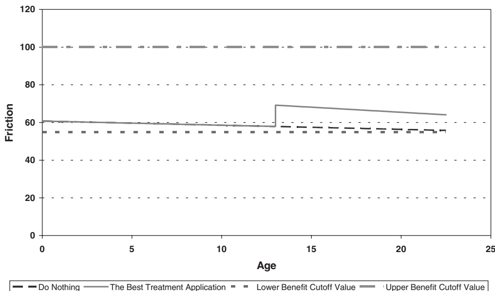
Figure 22. Friction versus age for the most appropriate application age of 13 years for Case Study 1—Arizona.
