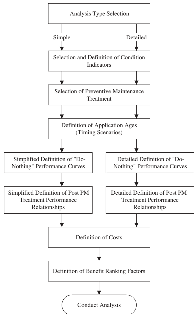
Figure 12. Outline of the data flow through the methodology.
