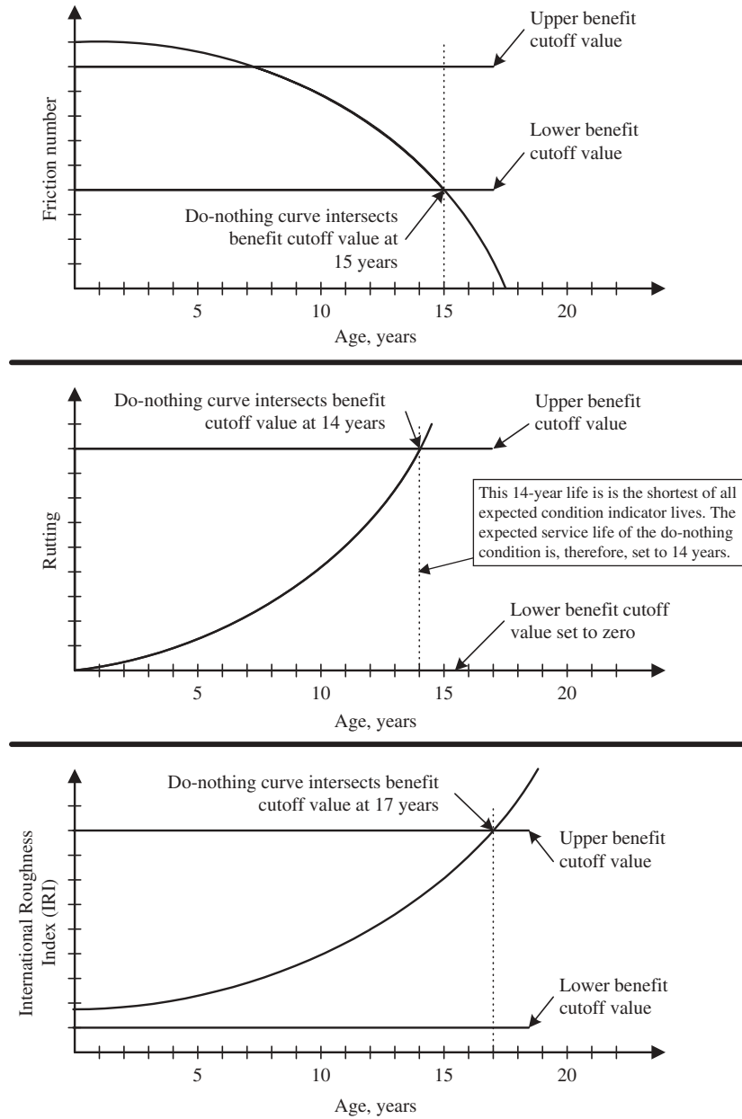
Figure 5. Determination of the overall do-nothing condition expected service life.
