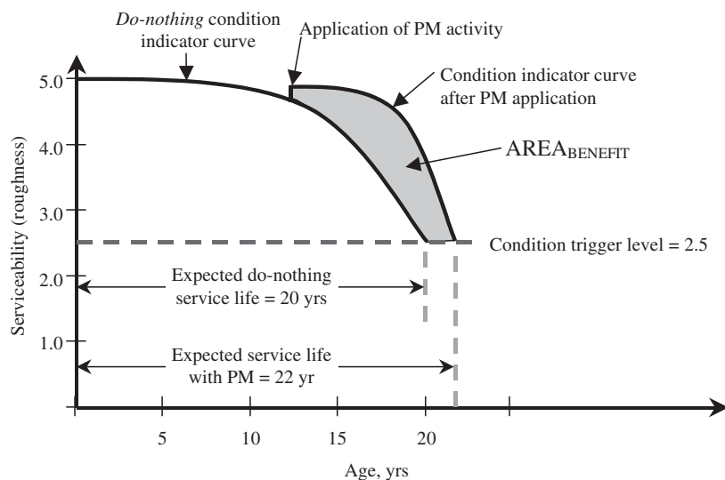
Figure D-2. Illustration of benefit associated with the application of a preventive maintenance treatment.
