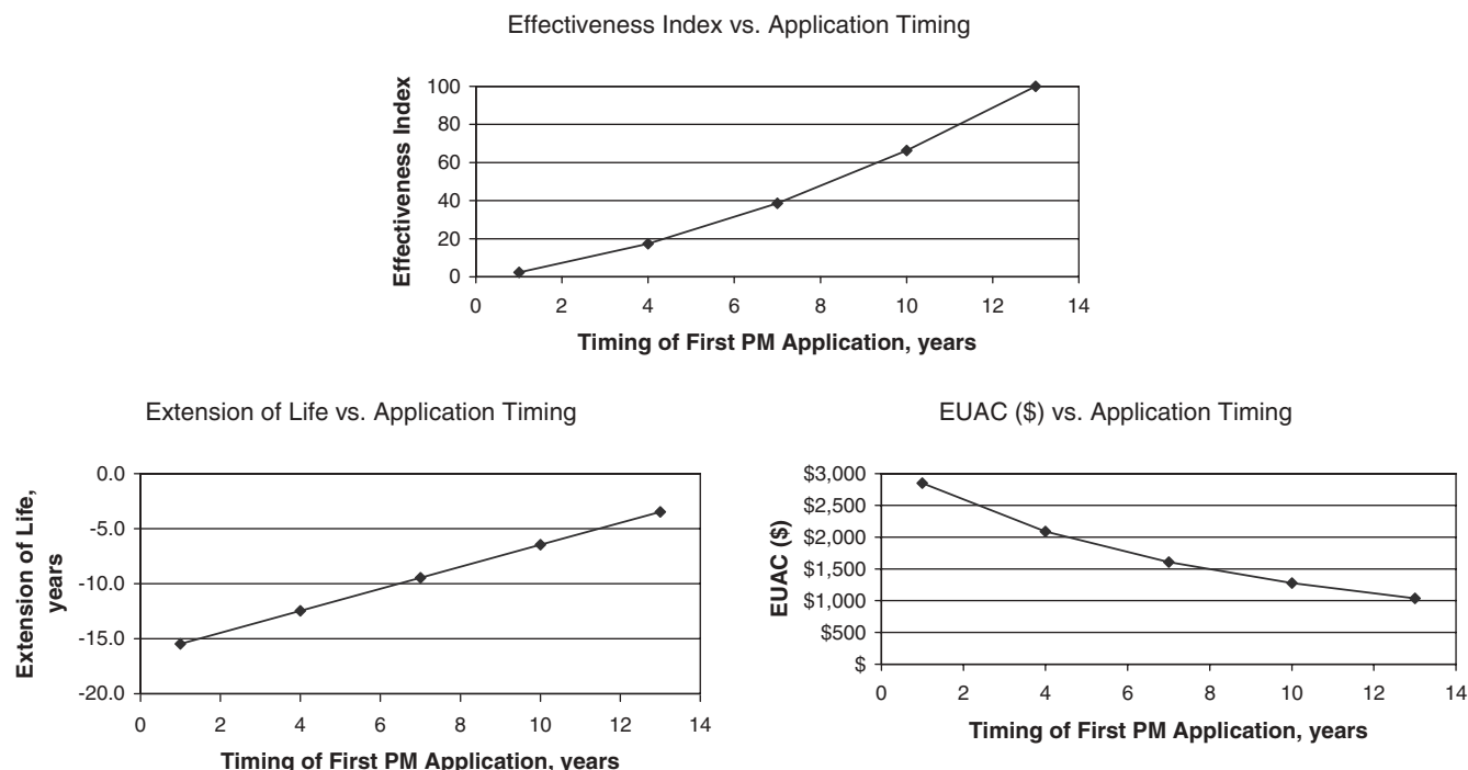
Figure 19. Results of the analysis for Case Study 1—Arizona.
