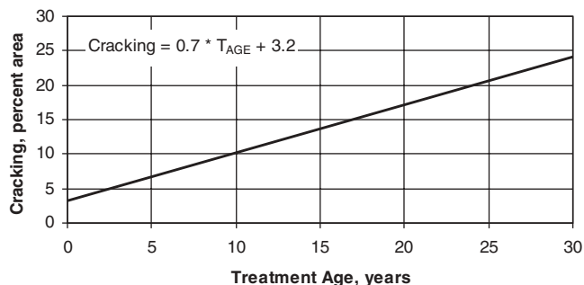
Figure 18. Assumed post-treatment seal coat cracking relationship for Case Study 1—Arizona.
